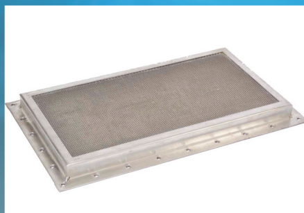
Exclusive honeycomb filter is available in choice of .5", .625", and 1" depths
